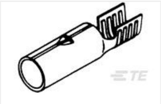
TE 产品编号42891-2 SHUR PLUG 180 RECEPTACLE 14-10 AWG TPBR
