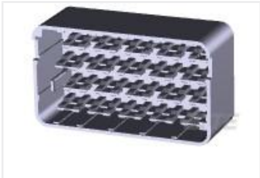
TE 产品编号178413-7 40P D.L.P FOR 120P ECU PLUG
