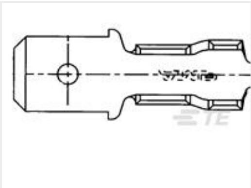
TE 产品编号41778 250 FASTON TAB 18-14 AWG TPBR
