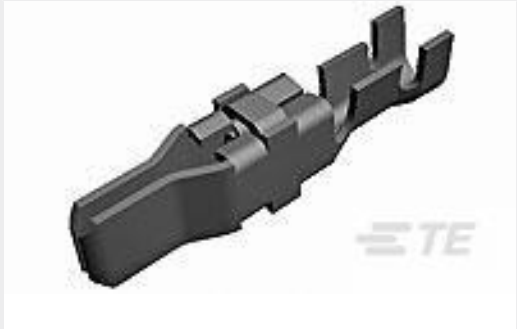
TE 产品编号1-66255-2 TYPE XII CONT ASY MALE
