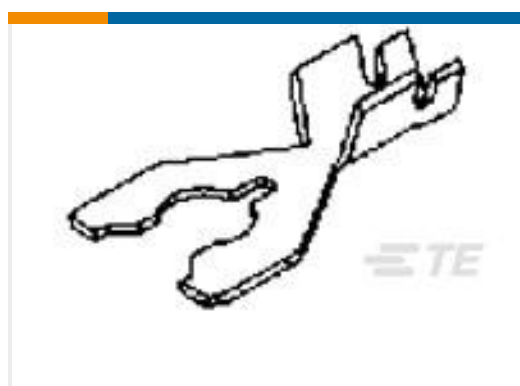
TE 产品编号60187-2 SPRING SPADE CRIMP 18-14 AWG TPBR
