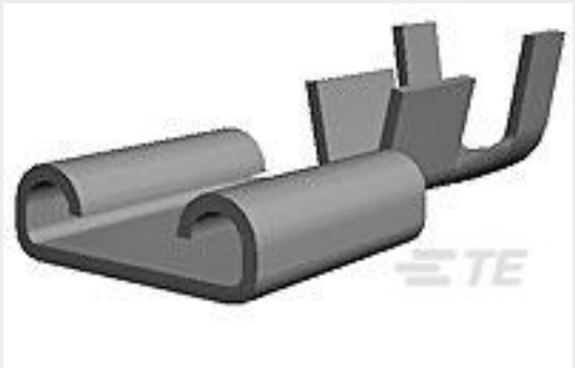
TE 产品编号170180-2 205 FASTON,REC.,18-14 AWG,TPBR
