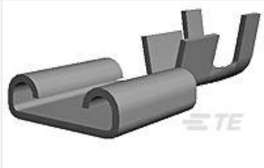
TE 产品编号170179-2 205 FASTON,REC.,18-14 AWG,TPBR
