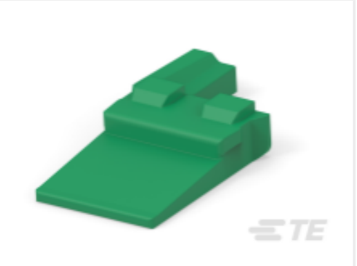
TE 产品编号W2PC WEDGE LOCK, 2P, REC, GRN, DT, C
