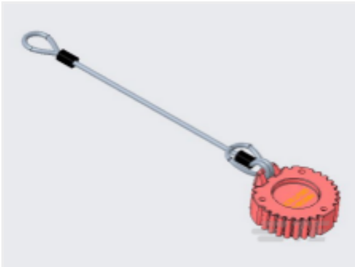
TE 产品编号HDC16-9-E004-L47N DUST CAP, 9P, REC, BLK, LANYARD, HD10
