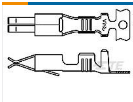
TE 产品编号643222-1 MINI-SPRING RECEPTACLE 20-16 AWG PTPBR
