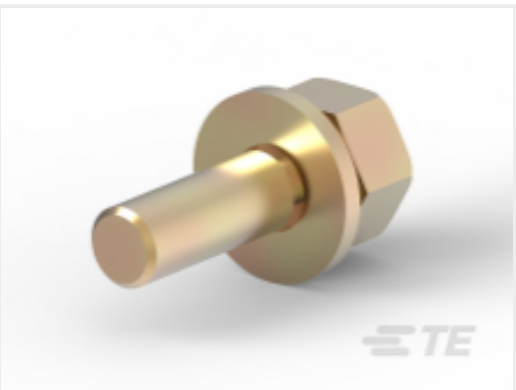
TE 产品编号HC5981 SCREW M6 x 20mm HEX HEAD CAPTIVE BATTER
