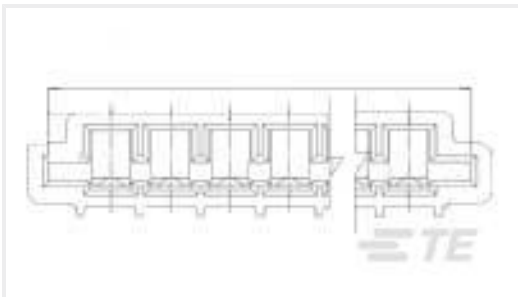
TE 产品编号5-487509-8 TRIOMATE ASY V 9P L=4.064,LDFR
