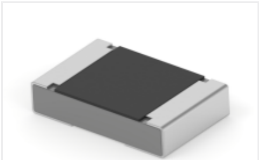
TE 产品编号5-2176482-8 RA73F 2A 200R 0.1% 5K RL
