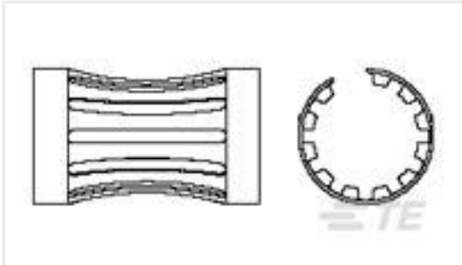
TE 产品编号1-192046-6 LAV 0.15mm(.006) GOLD
