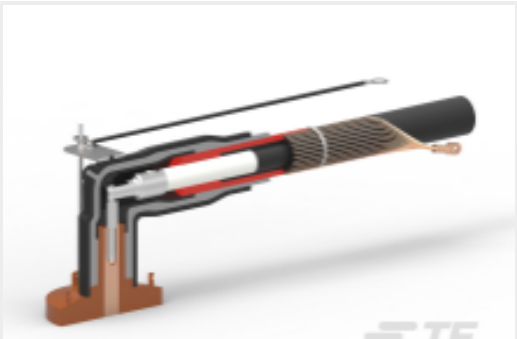
TE 产品编号EN3704-011 RSES-525B
