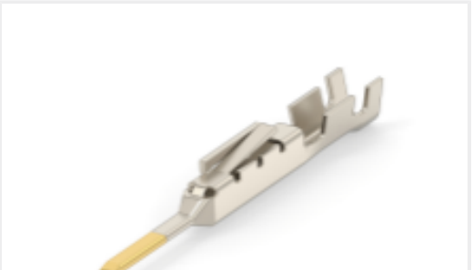
TE 产品编号CAT-D9934-A66 Contact: Component To Wire ; 5A, 28-18 wire size, gold plated
