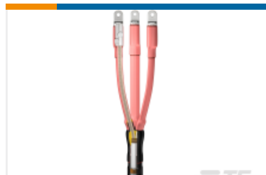
TE 产品编号A31452-070 GUST-12/70-120/800-L12
