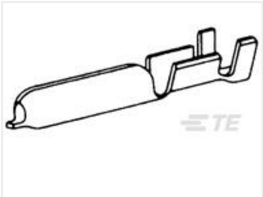
TE 产品编号62074-1 PIN .125 (3.17 MM) 24-20 AWG 0.42 BR
