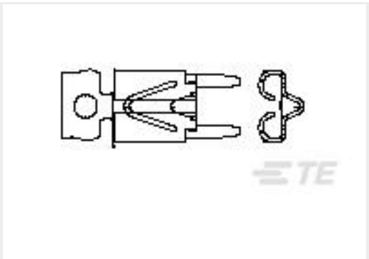
TE 产品编号63994-1 FASTON 205/250 PCB MOUNTED TPBR
