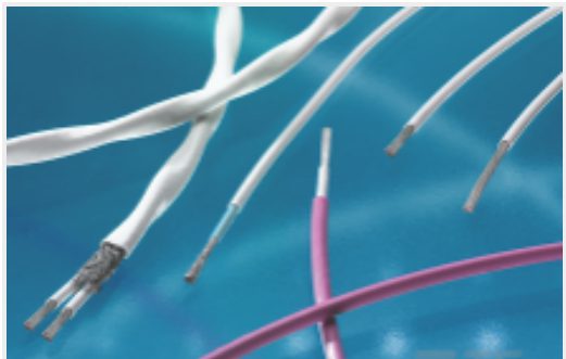
TE 产品编号 CAT-55M-SCH-TP Twisted Pair Cable: Silver Coated Cable, 450V Dual Wall
