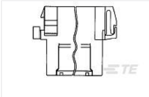
TE 产品编号929505-5 FF TAB HOUSING 2X7P
