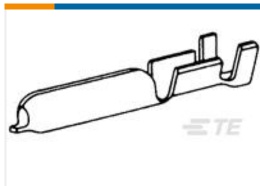
TE 产品编号62074-1 PIN .125 (3.17 MM) 24-20 AWG 0.42 BR
