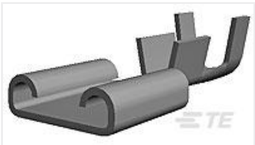
TE 产品编号4-160256-7 250 FASTON,REC.,17-14 AWG,SPBR
