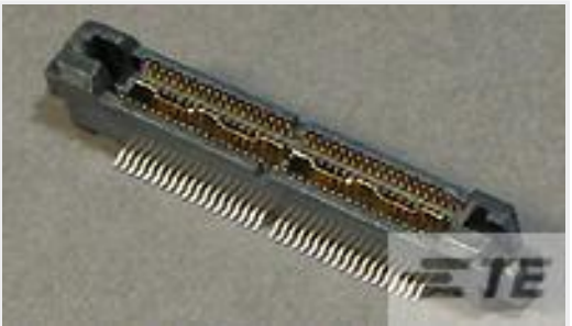
TE 产品编号5767056-2 MICT,260,PLUG,76,ASSY,PDNI
