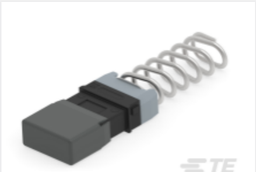
TE 产品编号2355002-1 MT Ferrule Kit,Plug,Without Pins,12-F, MM
