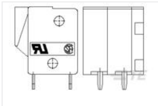
TE 产品编号1776259-2 2P Spring TB, 180deg, VT,5mm, Green
