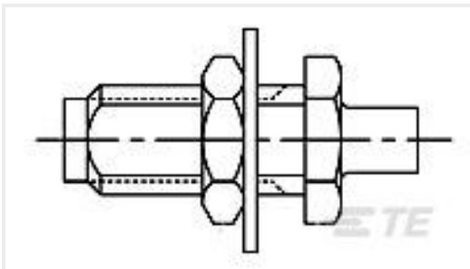
TE 产品编号1058990-1 OSMM STRAIGHT BLKHD CABLE 4004 7947 00
