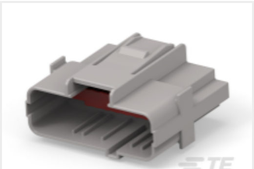
TE 产品编号2098380-8 20 POS HYBRID UNSEALED CAP KY-B ECP CLIP
