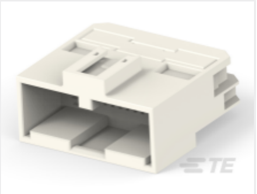
TE 产品编号2005395-1 025/090/110 HYB 18P CAP ASSY
