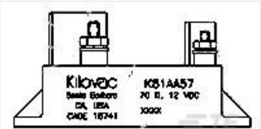
TE 产品编号1-1618241-8 K81AA57=RELAY, VACUUM, SPST-NO
