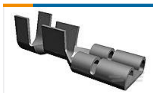
TE 产品编号63609-2 250 FASTON REC 22-18 AWG TPBR
