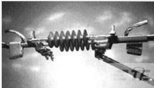
TE 产品编号83843-8 AMPACT ILD Replacement TAP 336.4
