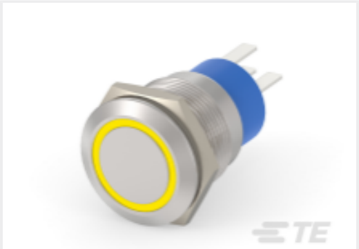
TE 产品编号3-2213767-1 AV19 SPL 3A MOVE RING LED YELLOW 24V
