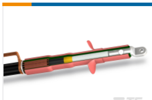
TE 产品编号C15907-064 POLT-42F/1XO-L16A
