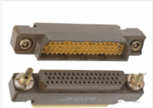
TE 产品编号ZPF00000000017884 FAST-E 03 F-X-A 00 B
