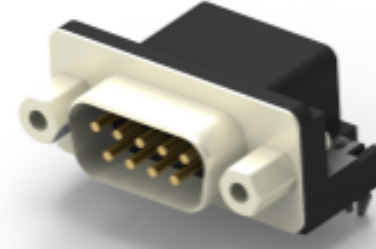
TE 产品编号2301843-2 AMPL PLUG HD20, R/A, 9P, B/L,4-40 S /LOCK
