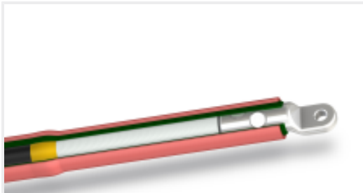
TE 产品编号C47372-064 GUST-12/25-50/800
