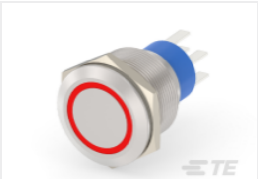
TE 产品编号6-2213772-7 AV22 DPL 3A MOVE RING LED RED 24V
