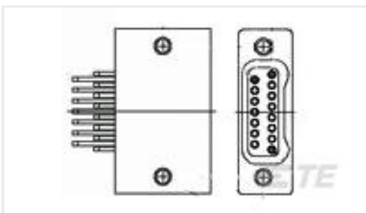
TE 产品编号7-1589483-3 STM065L2HN = SMT CONN
