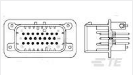
TE 产品编号776200-1 23POS,PIN DIA 1.3,HDR ASSY, 180DEG,COD 1
