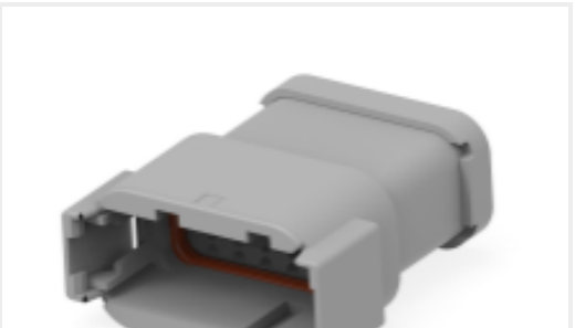
TE 产品编号DTM04-12PA-E003 REC, 12P, GRY, N, CAP, A
