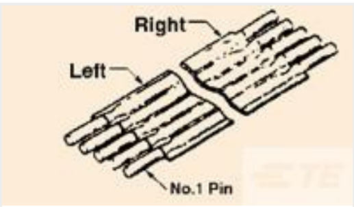
TE 产品编号5-1437142-9 FSN-22A-4=JUMPER, NOMEX
