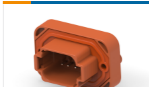
TE 产品编号DT13-08PD HDR, 8P, BRN, RA, NI/CU, D
