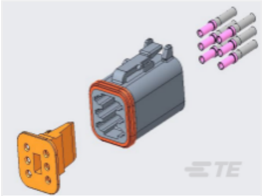
TE 产品编号DT06-6S-COMPLETE DT06-6S CON AND WEG
