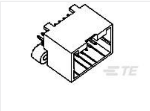
TE 产品编号174975-2 040 MLC CAP ASSY V 16P
