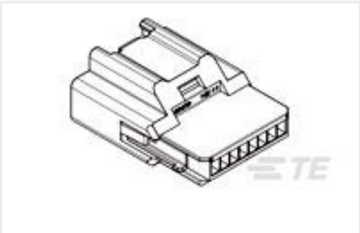
TE 产品编号9-1419166-0 GET;1X8 MALE CONNECTOR ASSY
