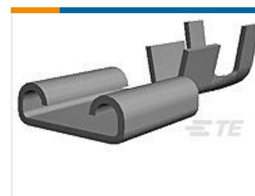
TE 产品编号160807-2 250 FASTON,REC.,20-16 AWG,BR
