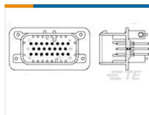
TE 产品编号1-776200-1 23POS,PIN DIA 1.3,HDR ASSY, 180DEG,COD 1
