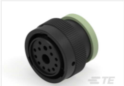
TE 产品编号HDP26-24-14SN-L017 PLG, 14P, BLK, N, RNG, 4/12/16, S
