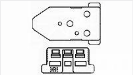
TE 产品编号316293-1 3.2 CLUSTER BLOCK HSG NATURAL
