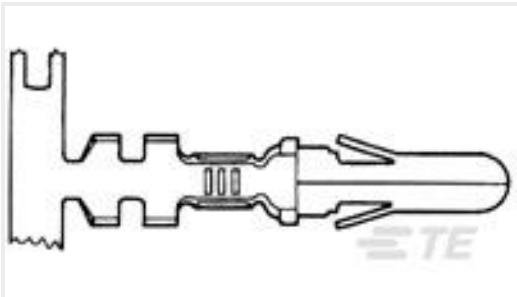
TE 产品编号350391-1 .140 DIA PIN 14-10 PTPBR L/P
