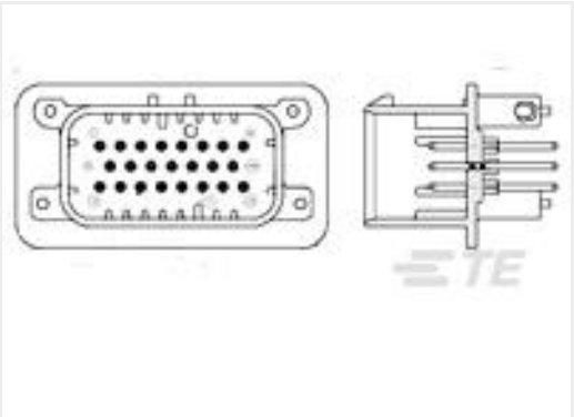
TE 产品编号776231-1 35POS,PIN DIA 1.3,HDR ASSY, 180DEG,COD 1
